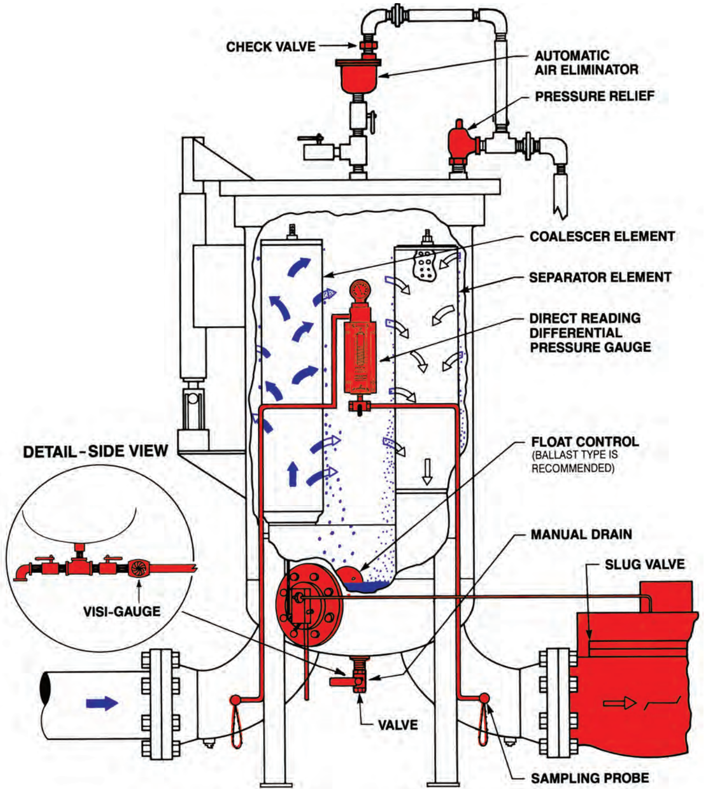
CUTAWAY—TYPICAL FILTER/SEPARATOR
